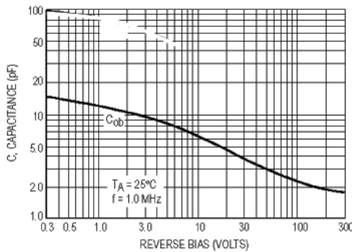
Figure 5. Capacitance
