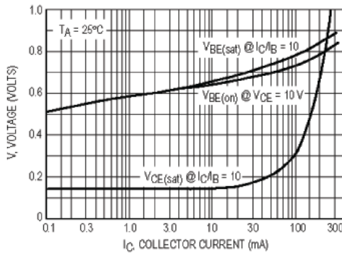
Figure 3. "On" Voltages
