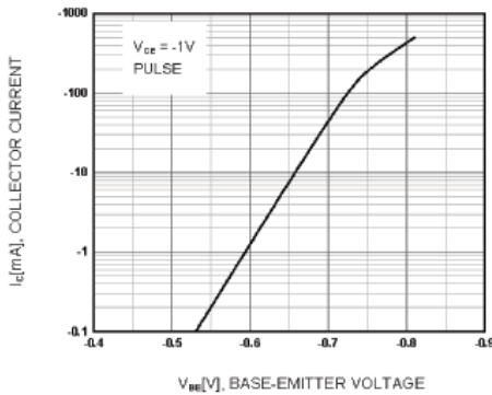
Figure 5. Base-Emitter On Voltage
