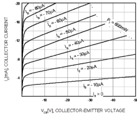
Figure 2. Static Characteristic
