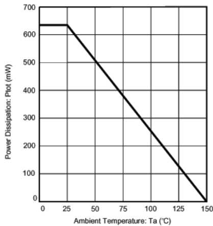
Power Dissipation vs Ambient Temperature
