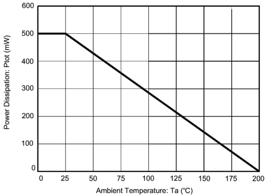
Power Dissipation vs Ambient Temperature
